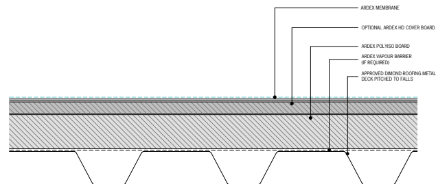
Warm Roof System - Metal Deck
