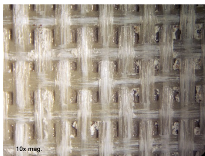
Mesh backed tile showing some degradation after several months immersed exposure and bonded to concrete with X77 adhesive.
